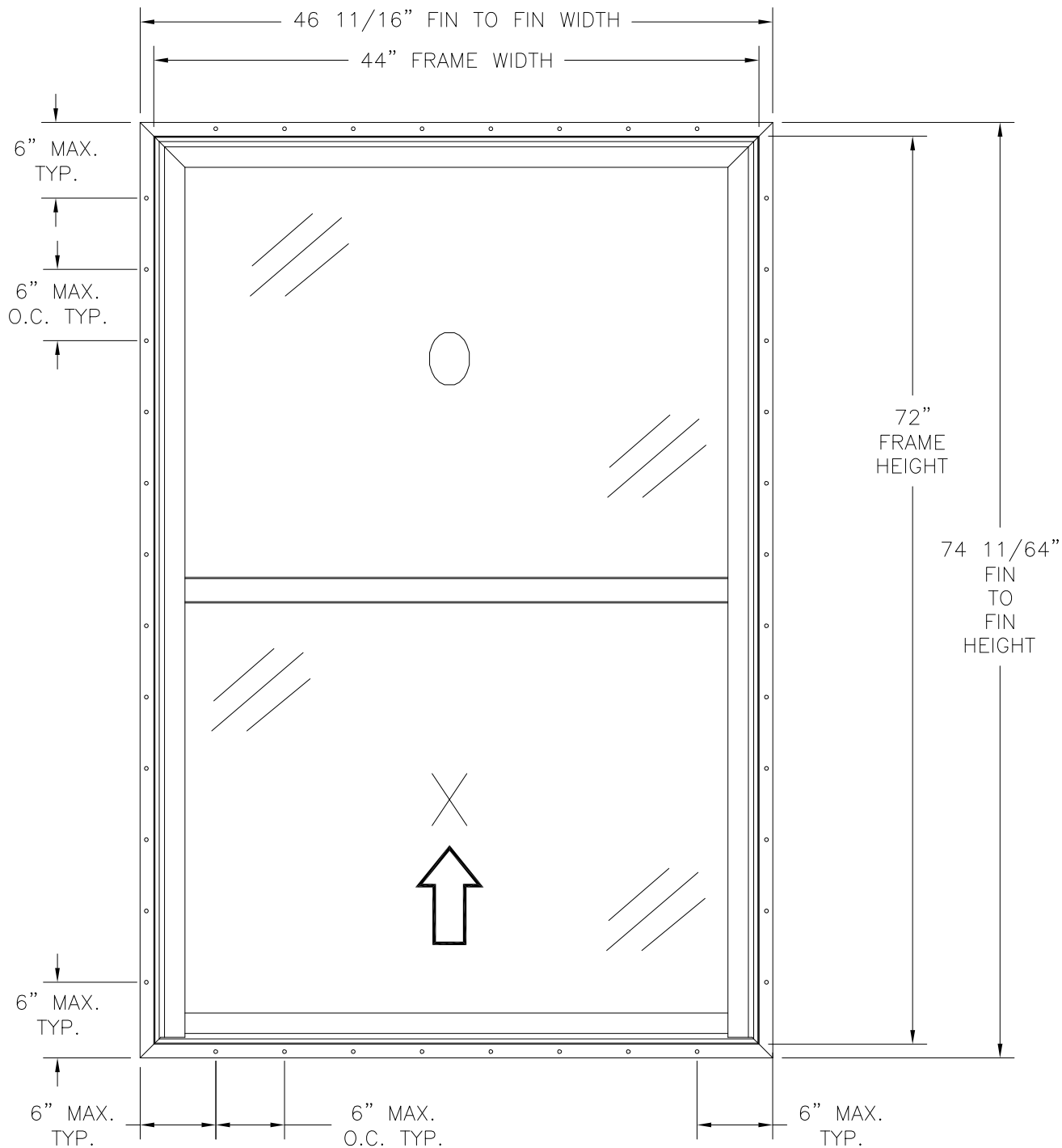
SHORELINE 1100 SH PVC SINGLE HUNG WINDOW EXTERIOR VIEW
