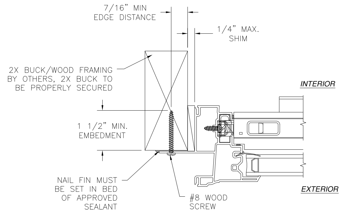
JAMB INSTALLATION 2X BUCK/WOOD FRAMING
