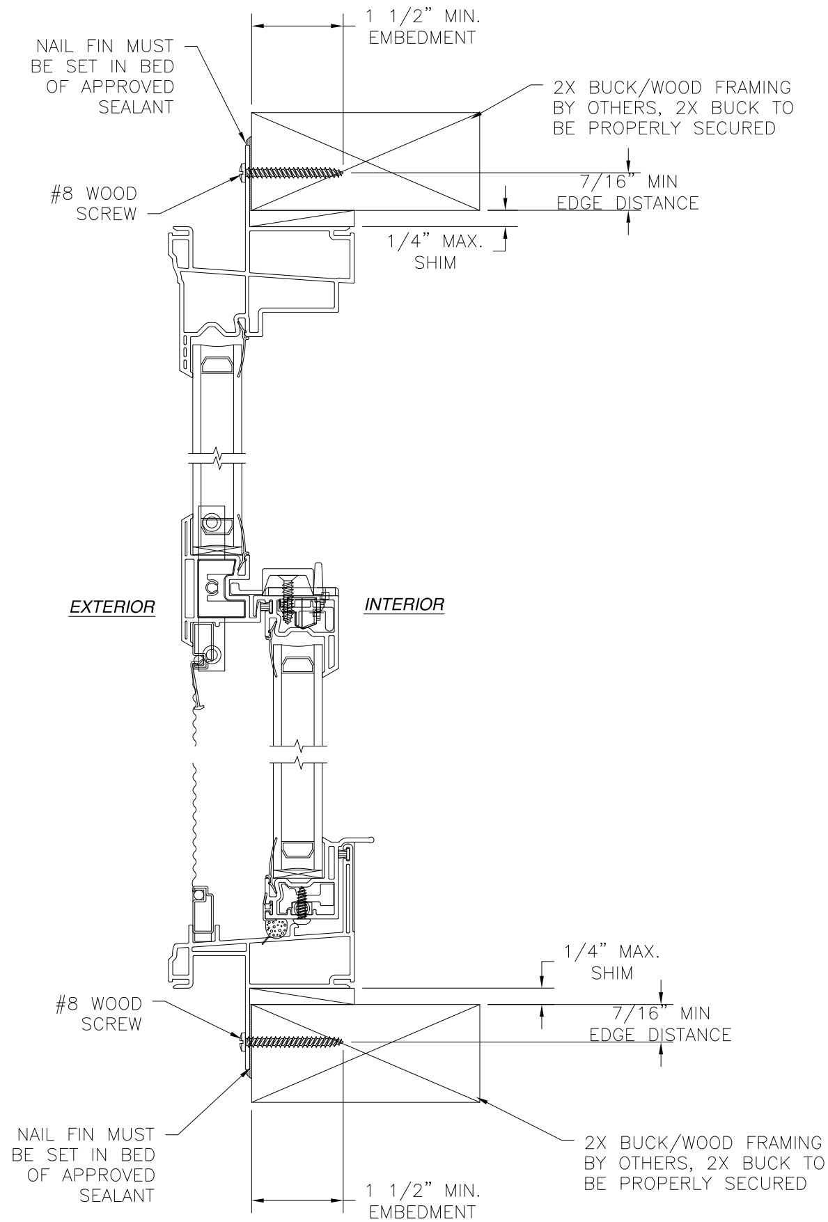
VERTICAL CROSS SECTION 2X BUCK/WOOD FRAMING INSTALLATION
